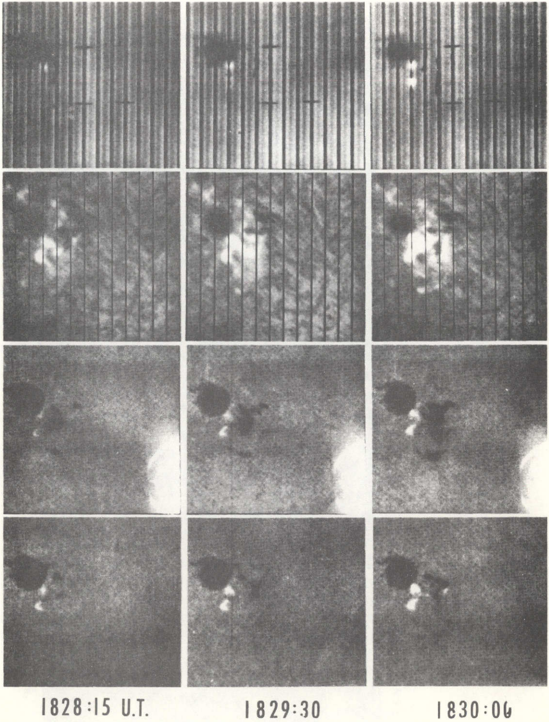
Figure XIII A. Beginning of Imp. IB flare on 5 September 1973 with the eruption of a filament.
