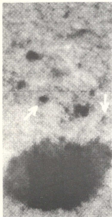
Figure IX. A small filamentary appendage accompanies a dying spot, while nearby a spot grows, with a D 3 event.
