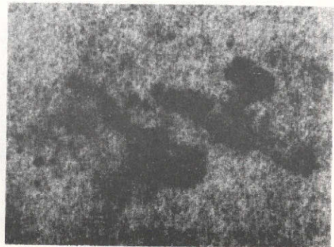
Figure IA. Two bright ribbons of D 3 emission in the Imp. IB flare of 11 April 1973, move apart at 8 km/sec. D 3 absorption obscures underlying sunspots.
